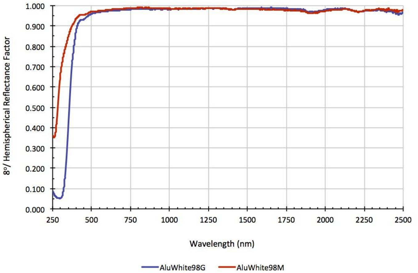
AluWhite 8°/Hemispherical Reflectance Factor
