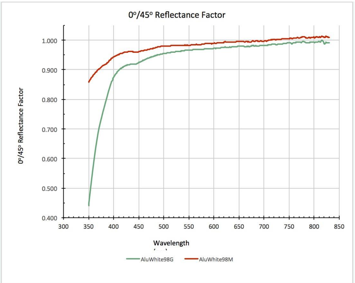
AluWhite 0°/45° Reflectance Factor
